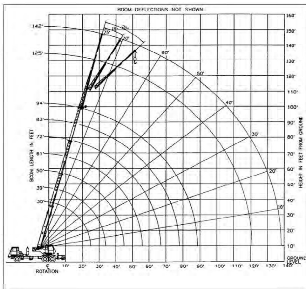
Range Diagram (30' - 94' boom)
