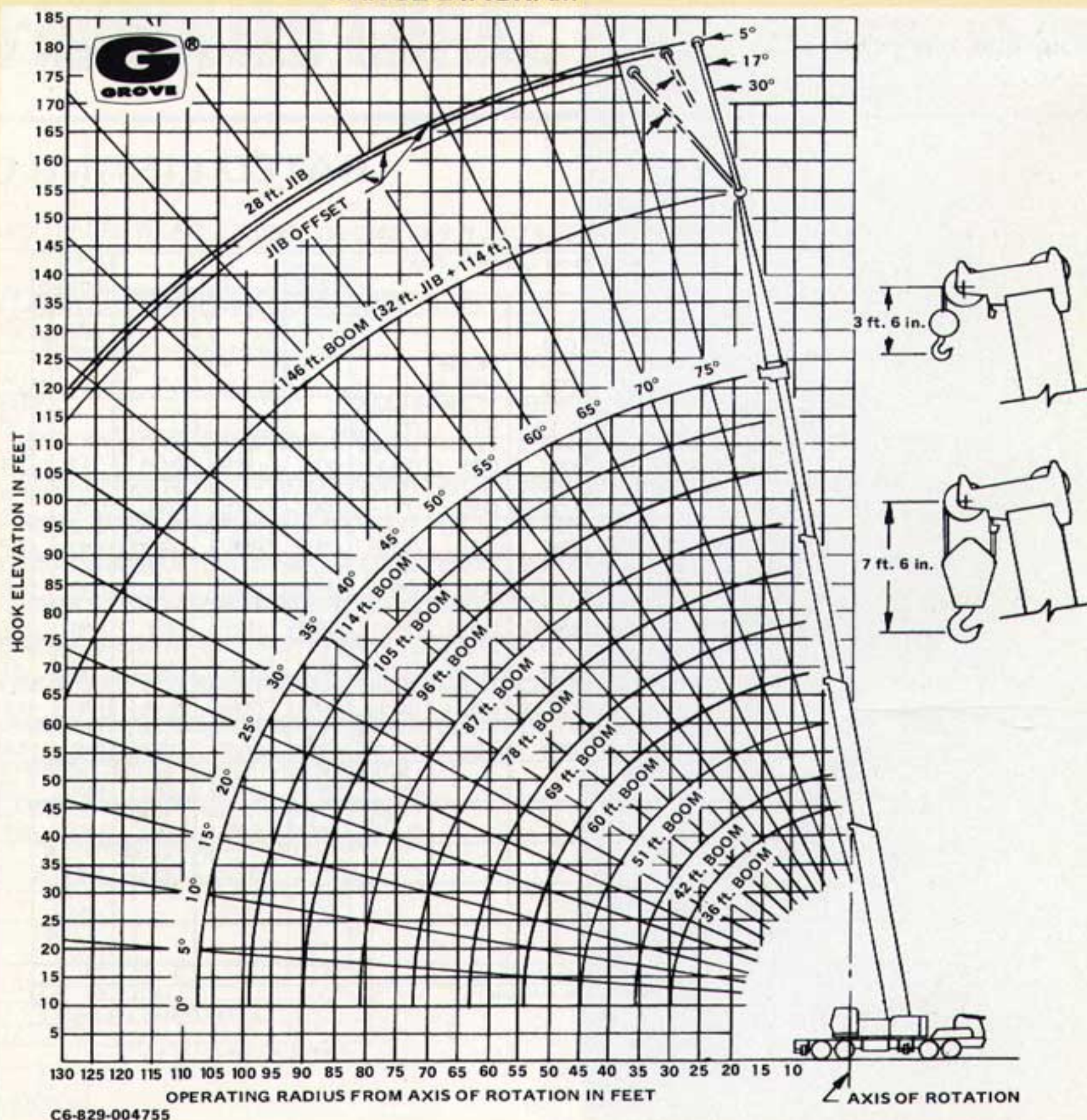
RANGE DIAGRAM
