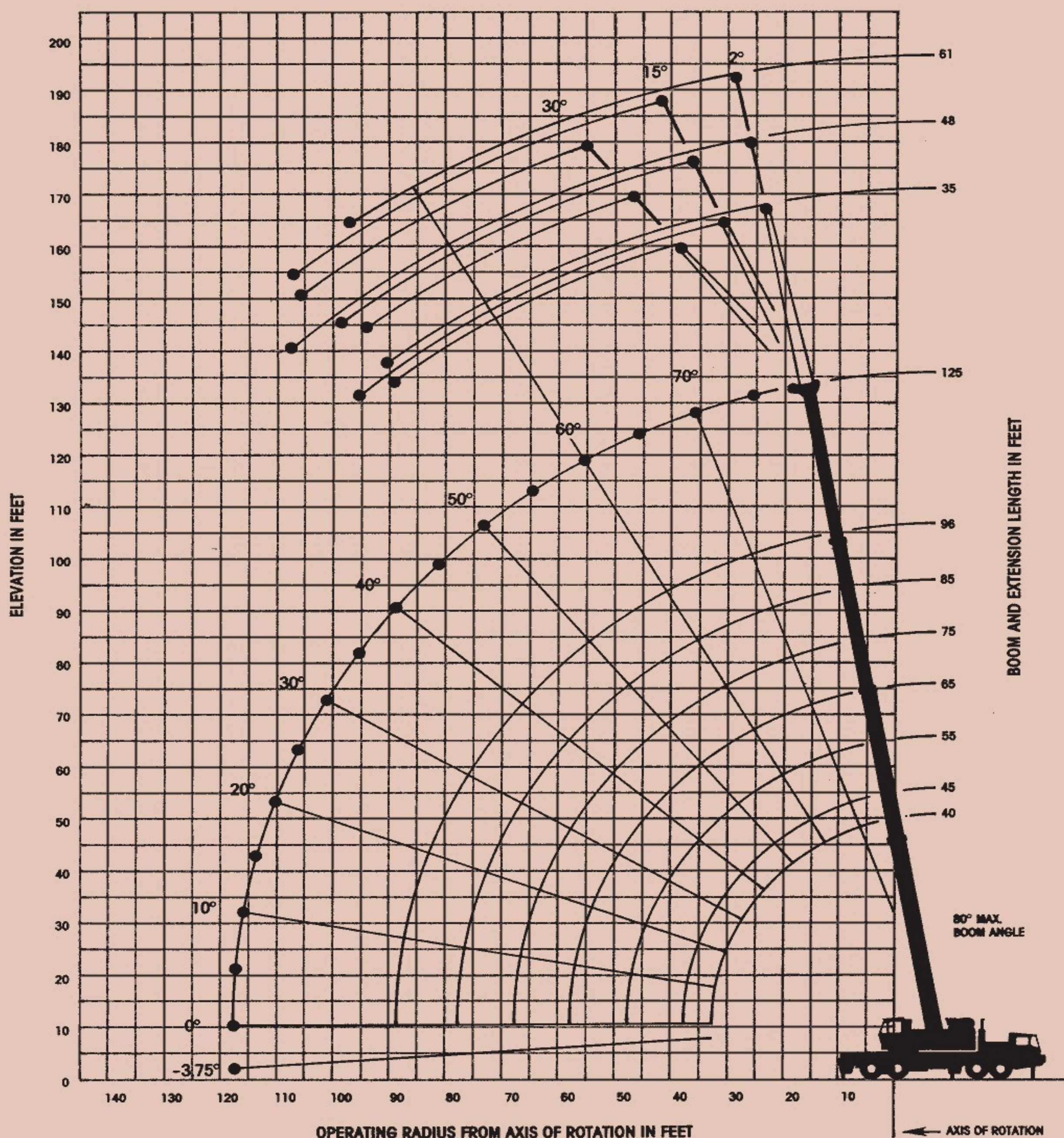
RANGE DIAGRAM (UNLADEN BOOM)
