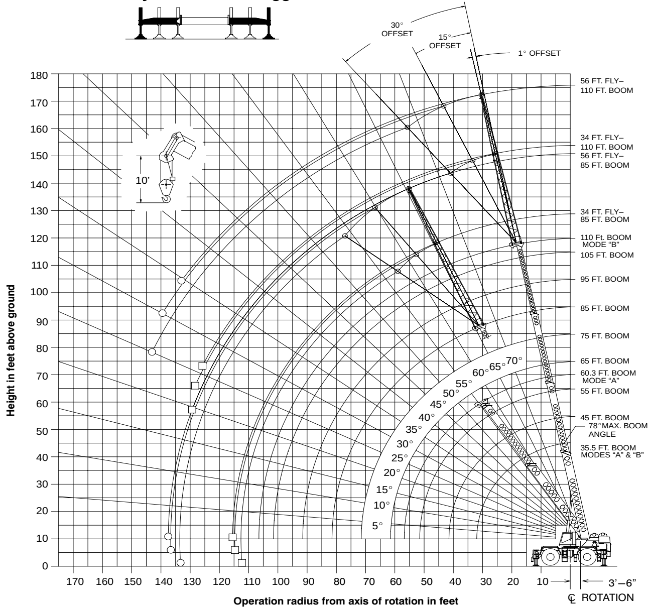
Working Range Diagram On Fully Extended Outriggers
