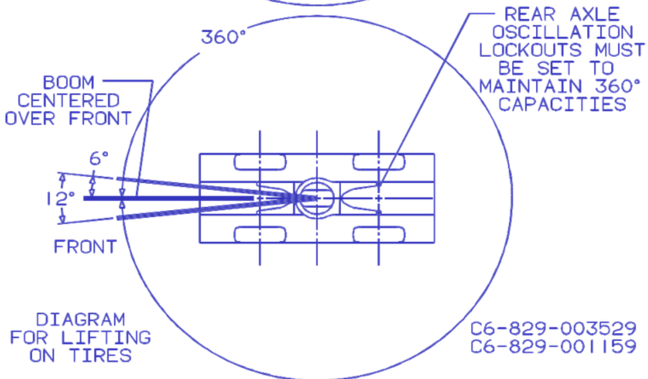
DIAGRAM FOR LIFTING ON OUTRIGGERS
