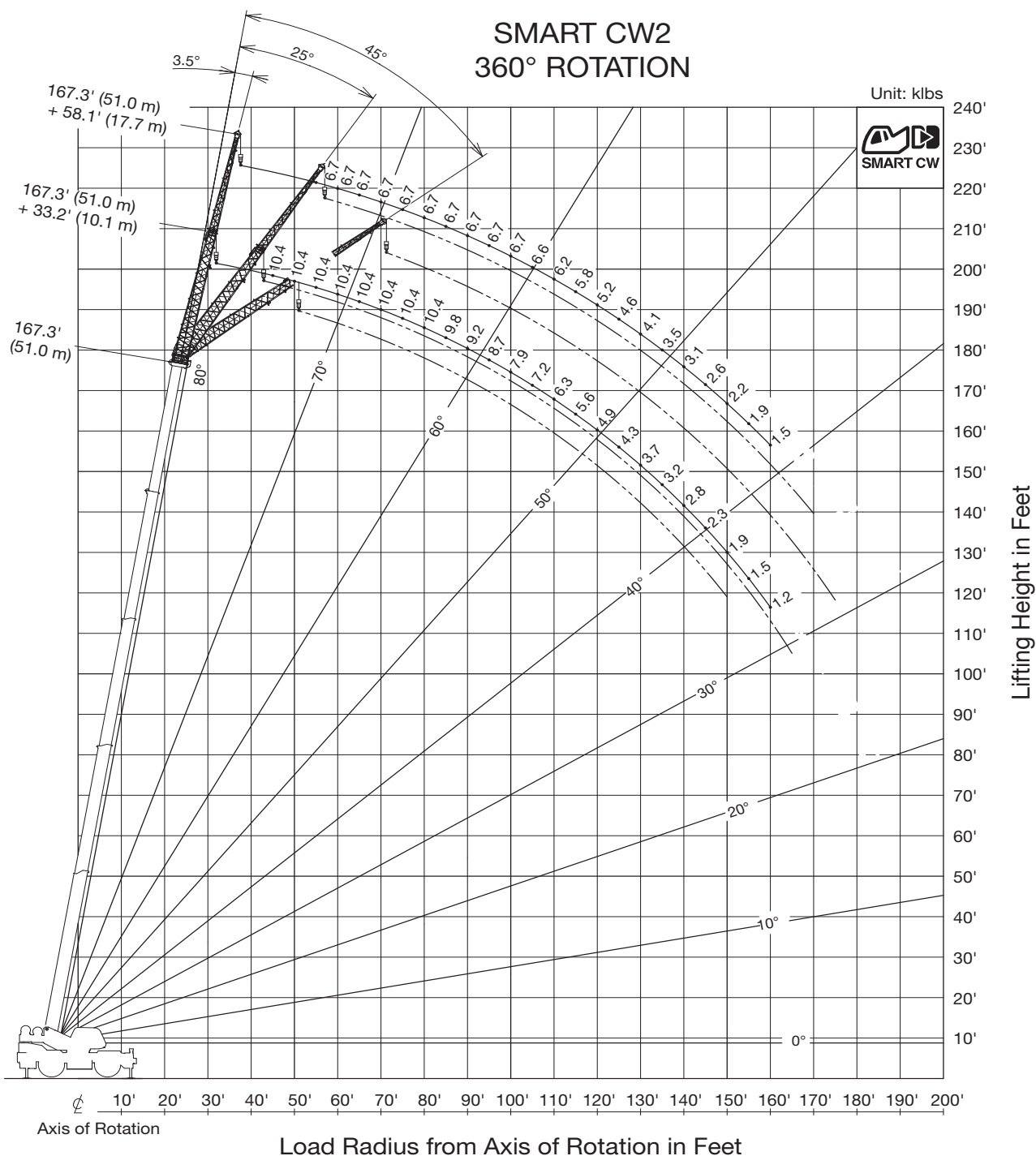
JIB
