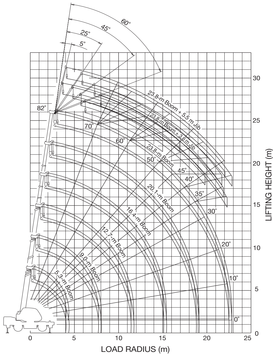
JIB
