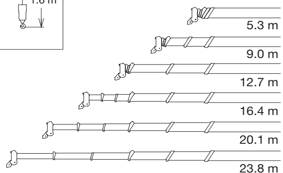
Boom Length
